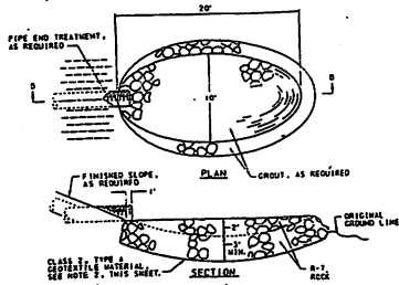
ROCK BASIN DETAILS NOT TO SCALE
