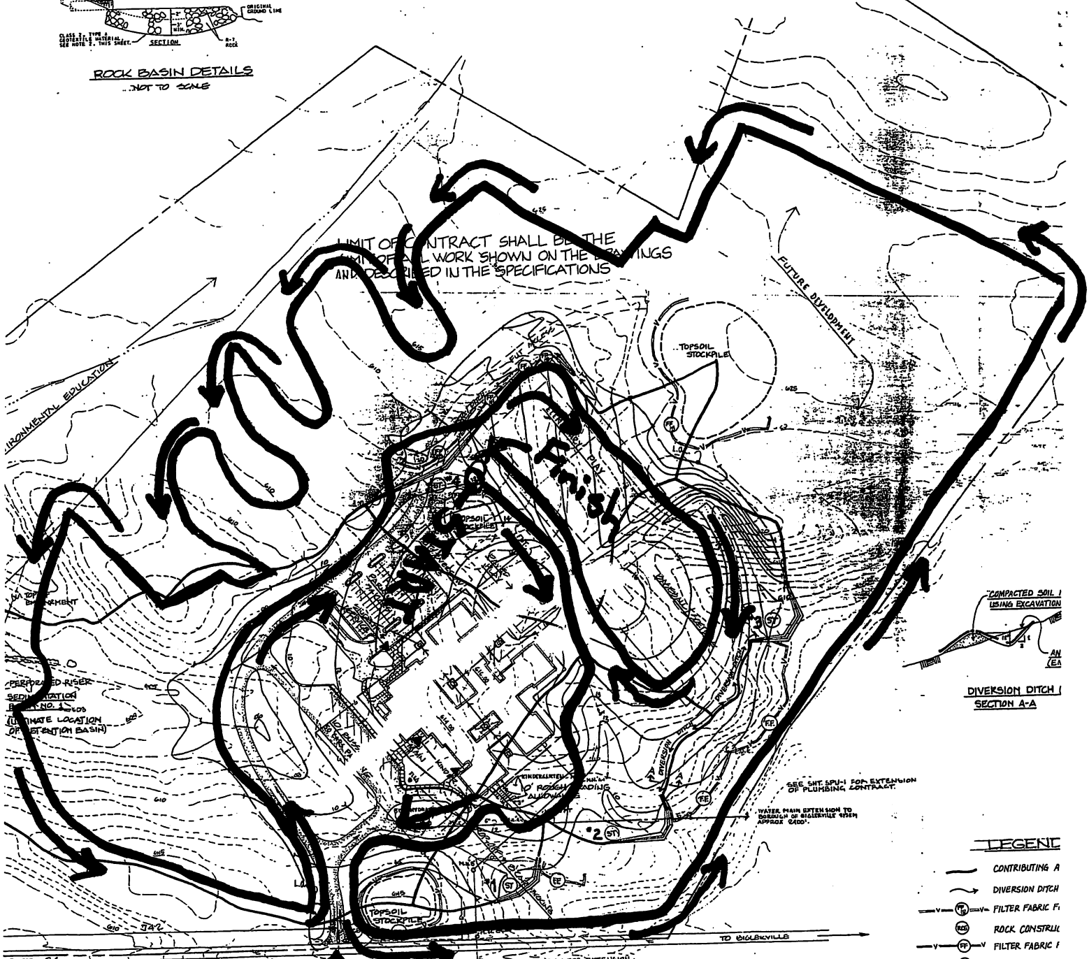
ROCK CONSTRUCTION ENTRANCE NOT TO SCALE
